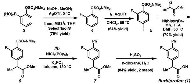
Figure 2. Synthesis of flurbiprofen using orthogonal cross-couplings.
