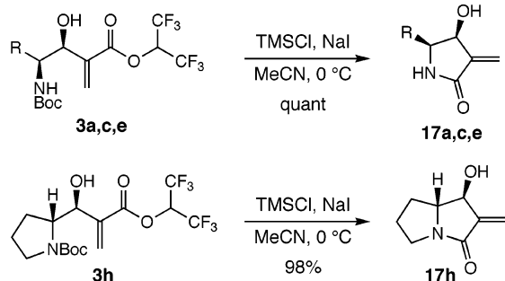
Scheme 4. Synthesis of Functionalized Pyrrolidinones
