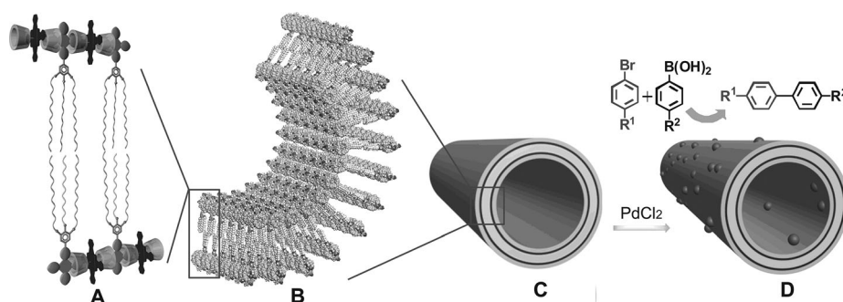
Scheme 2. Schematic representation of the tubular self-assembly. A) Building blocks of 1 and 2 in the formation of the nanotube wall. B) Self-assembly of the nanotube wall. C) Supramolecular nanotube with a bilayer array of 1·2 complex. D) Test reaction catalyzed by Pd@NT.
