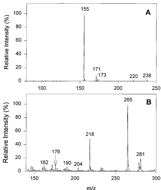
Figure 3. API-MS spectra of irradiated \text{CH}_3\text{ONO}/\text{NO}/\text{n-decane}/\text{air} mixtures. (A) Positive ion mode with protonation by \text{H}_3\text{O}^+(\text{H}_2\text{O})_n ions. (B) Negative ion mode using \text{NO}_2^- adduct ions. See text for assignments of the observed ion peaks.
