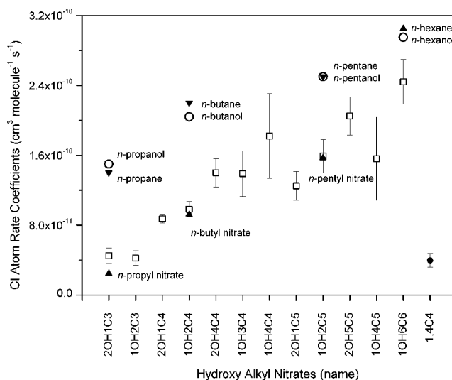
Figure 4. Schematic presentation of the Cl atom rate coefficients of the hydroxyalkyl nitrates and dinitrate and a comparison with their corresponding alkyl nitrates, alkanes, and alcohols: (□) hydroxyalkyl nitrates; (▼) n -alkanes; (▲) alkyl nitrates; (○) alcohols; (●) dinitrate. 22,29,36–38
