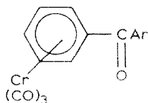
(9a, Ar = Ph ;
