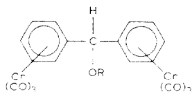
(5a, R = CH 3 )
