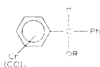
(4a, R = CH 3 )
