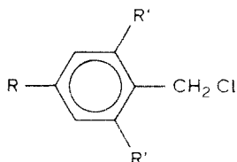
(8a, R = R' = H ;
