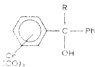
(6a, R = CH 3 )
