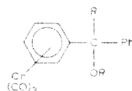
(7a, R = CH 3 )
