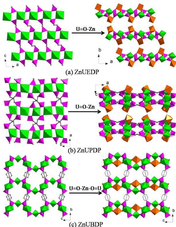
Figure 2. Uranyl phosphonate partial structures connected by zinc-centered polyhedra via CCIs to form the whole structures of ZnUEDP (a), ZnUPDP (b), and ZnUBDP (c).
