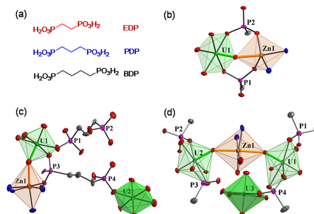
Figure 1. Diphosphonate ligands (a) and the connection modes of uranium and zinc atoms in \text{ZnUEDP} (b), \text{ZnUPDP} (c), and \text{ZnUBDP} (d).
