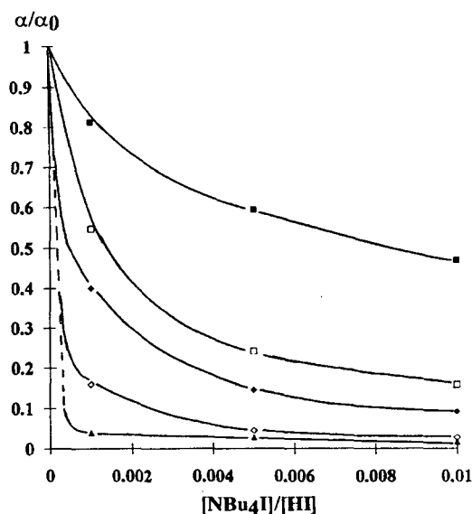
Figure 4. Variation of a/a_0 with [NBu_4I]/[HI] ratio for different hypothetical K_D values assuming C^* = 10^{-4} [HI] M; K_{NBu_4I} = 8 \times 10^{-5} M; 14 [HI] = 0.01 M. K_D = (■) 5 \times 10^{-5} ; (□) 1 \times 10^{-5} ; (◆) 10^{-6} ; (◇) 1 \times 10^{-6} ; (▲) 5 \times 10^{-7} .
