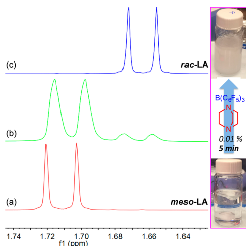
Figure 1. Left: NMR spectra (CDCl 3 ) of the methyl region of: (a) pure meso -LA; (b) meso -LA/ rac -LA (90/10) from NatureWorks; and (c) isolated pure rac -LA from epimerization of meso -LA. Right: pictorial representation of fast epimerization of meso -LA to rac -LA (which precipitates out of solution) by DABCO/B(C 6 F 5 ) 3 (2.88 g scale, 2.0 M in toluene, 5 min, 95.4% conversion).
