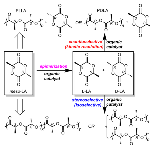
Scheme 1. Proposed New Strategy for Utilization of meso -LA
