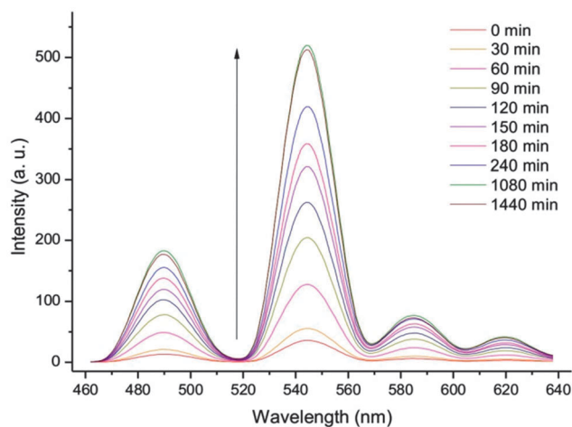
Scheme 4 Luminescence intensity of Vs4 ( C_{\text{DOPC}} = 5 \text{ mM} , C_{\text{Chol}} = 0.75 \text{ mM} , C_{\text{Tb}^{3+}} = 0.25 \text{ mM} ) is increasing in the presence of DHNDhn ( 12.5 \text{ }\mu\text{M} ) and lipase ( 50 \text{ mg L}^{-1} ) over 24 h.
