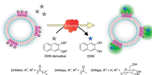
Scheme 3 Lipase conversion of naphthalene-2,3-dihydroxyesters ( 12.5 \text{ }\mu\text{M} ) into DHN leads to an increase of the terbium luminescence intensity.
