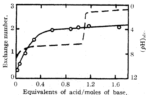
Fig. 2.—The rate of exchange of dimethylaniline in deuteroalcohol with varying amounts of sulfuric acid. The dotted line indicates the estimated (\text{pH})_{\text{alc.}} .
