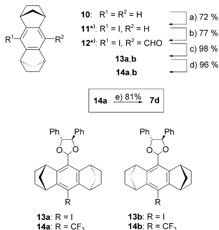
Scheme 4. Preparation of the trifluoromethylated aldehyde 7d from the octahydro-bis-methano-anthracene 10 . *: racemic mixture; a) \text{PhI}(\text{OAc})_2 , \text{I}_2 ; b) \text{SnCl}_4 , \text{Cl}_3\text{CHOCH}_3 ; c) ( R,R )-hydrobenzoin, PPTS; d) \text{CF}_3\text{-TMS} , \text{CuI} , \text{KF} ; e) aq. \text{HCl} , (\text{CH}_2\text{O})_n .
