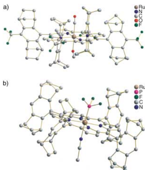
Figure 1. X-ray crystal structure of the ruthenium porphyrin a) 2d and b) chiral ruthenium- \text{PF}_3 -porphyrin 2e . a) The upper axial coordination site is occupied by a CO molecule, whereas the lower one carries a methanol molecule. b) The upper axial coordination site is occupied by a \text{PF}_3 molecule, whereas the lower one carries an acetonitrile molecule.
