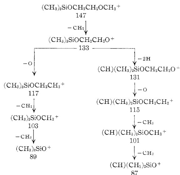
SCHEME I POSSIBLE FRAGMENTATIONS OF THE PRODUCT FROM THE REACTION OF 2-METHOXYETHANOL
