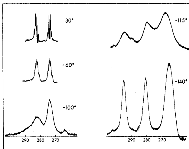
Figure 1. The 100-MHz ^1\text{H} nmr spectra of the \text{N}(\text{CH}_3)_2 region of \text{CF}_3\text{P}[\text{OSi}(\text{CH}_3)_3]\text{N}(\text{CH}_3)_2 . The scale gives shifts in hertz from external TMS. The spectra were obtained from approximately 20% solutions in the mixed solvent \text{CFCl}_3\text{--CF}_2\text{Cl}_2 . Increased spectral amplitudes were used for the low-temperature spectra ( -100 to -140^\circ ).
