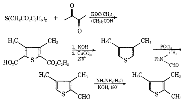
Scheme III. Preparation of 2,3,4-Trimethylthiophene
