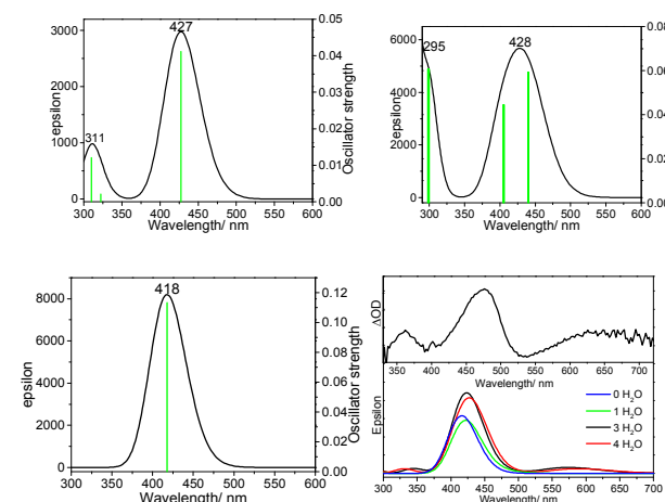
Figure 4. Shown are the computed electronic spectra of the m -dimethylamino phenoxy radical (top left), the triplet m -dimethylamino phenyloxenium ion 32 (top right) and the singlet m -dimethylamino phenyloxenium ion 12 (bottom left) from TD-B3LYP/6-311G(2d,p) calculations. Bottom right of the figure shows the experimental UV-vis spectrum at 19 ps after the pulse and the computed spectrum of the singlet
