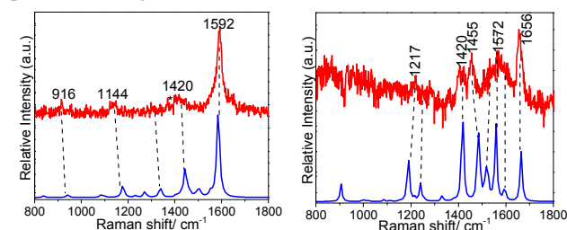
Figure 6. Left: comparison of the ns-TR 3 spectrum obtained at
