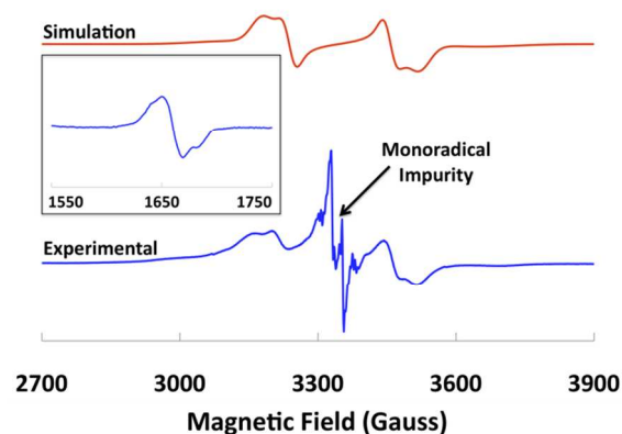
Figure 8. X-band EPR spectrum of 1 irradiated in EtOH glass at 4 K using a mercury lamp source delivered via a fiber optic cable into the cavity. Triplet simulation parameters: D = 280\text{ Gauss} ( |D|/hc = 0.026\text{ cm}^{-1} ), E/|D| = 0.075\text{ Gauss} ( 7.0 \times 10^{-6}\text{ cm}^{-1} ). Inset: \Delta m_s = 2 transition.
