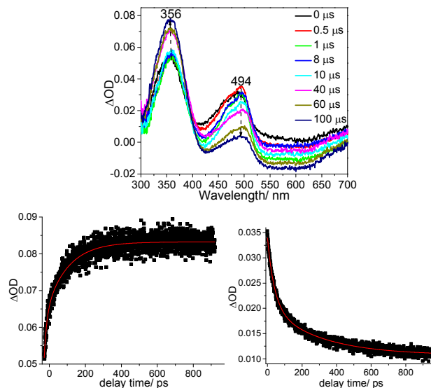
Figure 7. Top: ns-TA spectra from 0 \mu s to 100 \mu s produced in a MeCN:H 2 O 1:1 solution acquired after 266 nm irradiation of the initial precursor compound are shown. See text for more details. Bottom: The temporal dependences of the transient absorption intensity of initial compound in a MeCN:H 2 O 1:1 mixed solution at 356 (left) nm and 494 nm (right) are shown. The solid red line indicates fittings using a bi-exponential function.
