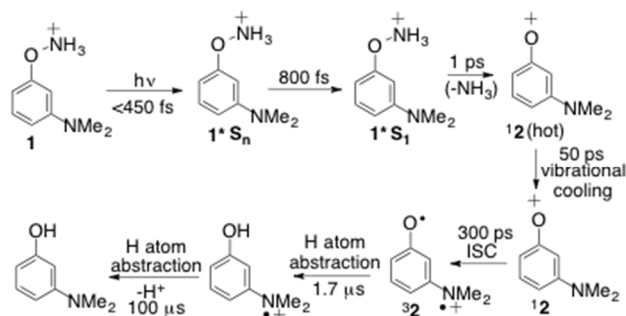
Scheme 1. Proposed mechanistic pathway based on piecing together the spectroscopic data.
