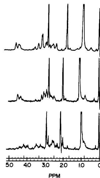
Figure 2. Eu(fod) 3 -shifted 1 H NMR spectra of trans -3 (top), trans -4 (middle), and cis -4 (bottom).
