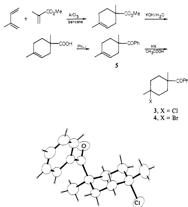
Figure 1. ORTEP 53 drawing of the molecular structure of trans -3. The thermal ellipsoids have been scaled to include 50% probability; the thermal parameters for H atoms have been set to an arbitrary small value.
