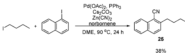
Scheme 1. Initial Conditions for Intermolecular Reaction
