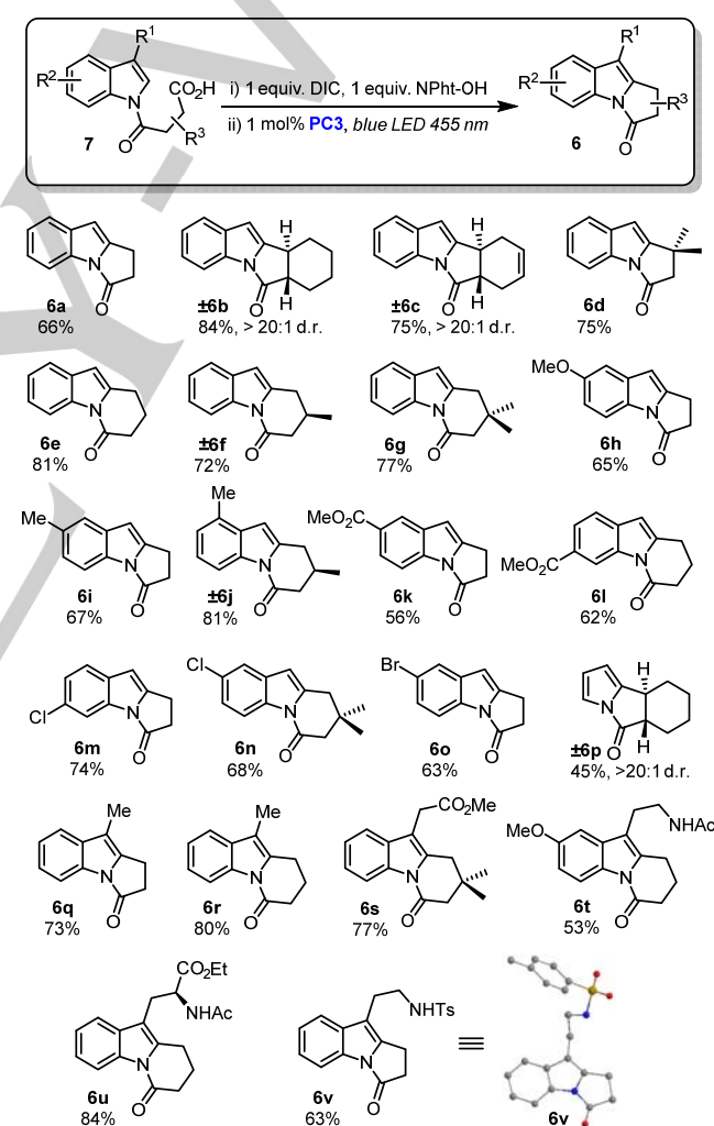
Scheme 3. Scope of the reaction.
