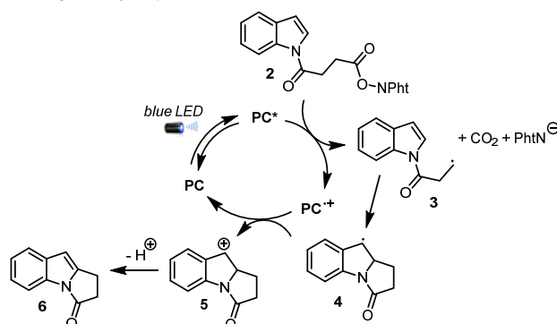
Scheme 2. Catalytic cycle of the envisaged strategy.
