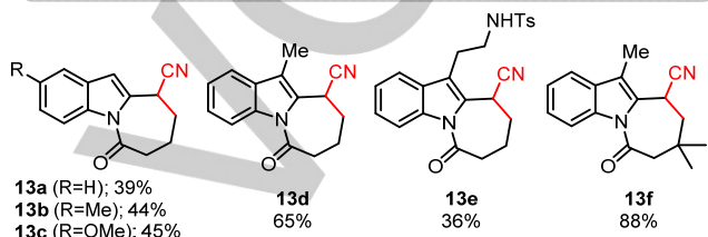
Scheme 5. Synthesis of azepinoindolones.
