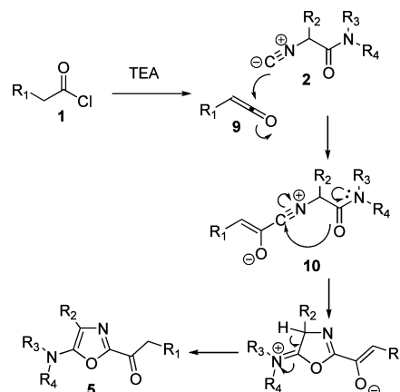
Scheme 6. Proposed Mechanism for the Synthesis of 2-Acyl-5-aminooxazoles
