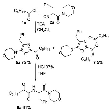
Scheme 2. Synthesis of 2-Acyl-5-aminooxazole 5a and Its Subsequent Acid Hydrolysis to \alpha -Ketoamides 6a
