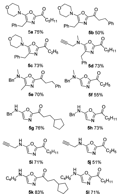
Figure 2. Synthesized 2-acyl-5-aminooxazoles.
