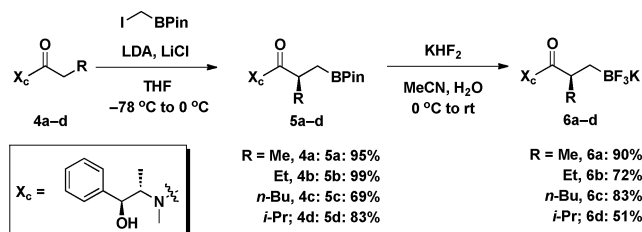
Scheme 3. Preparation of \alpha -Chiral \beta -Trifluoroboratoamides
