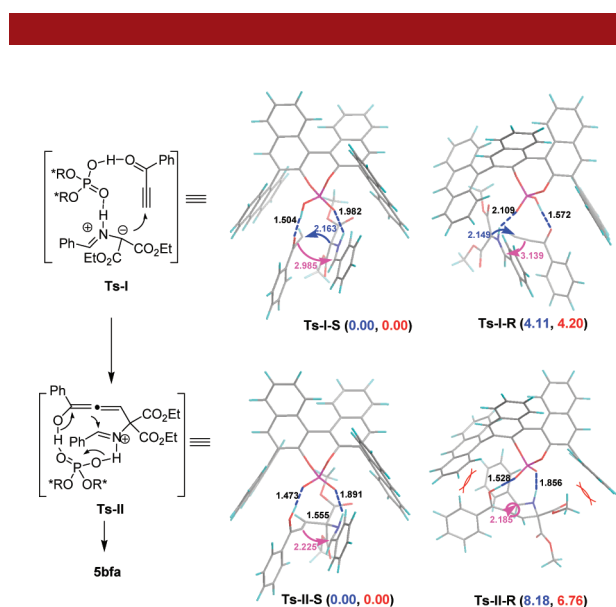
Figure 1. B3LYP/6-31G* optimized transition state structures and partial crucial bond length parameters in angstrom, relative energies in enthalpy (blue) and Gibbs free energy (red), and reaction mechanism.
