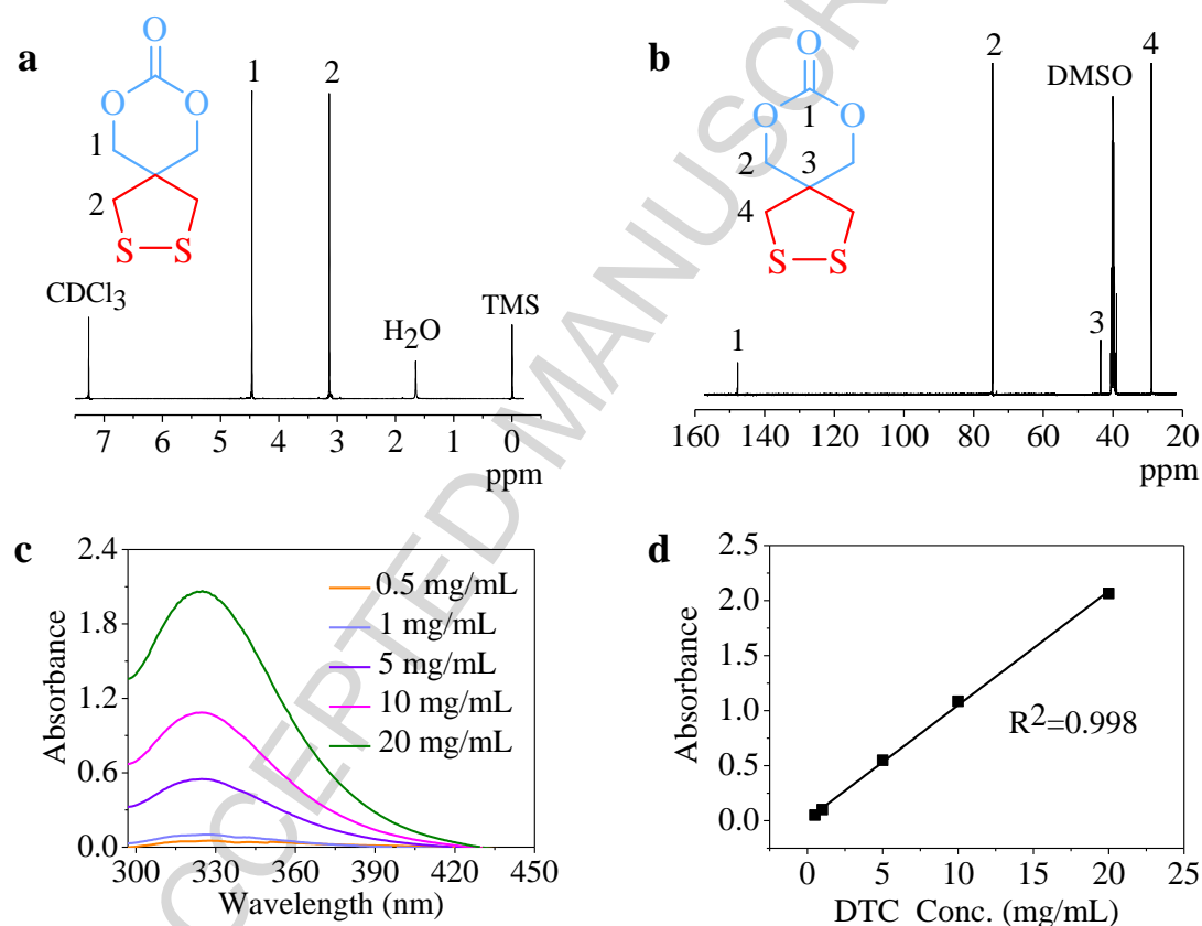
Fig. 1. Characterizations of DTC. (a) ^1\text{H} NMR Spectrum (400 MHz, \text{CDCl}_3 ) of DTC. (b) ^{13}\text{C} NMR Spectrum (100 MHz, \text{DMSO}-d_6 ) of DTC. (c) UV Spectrum of DTC in DMF at concentrations ranging from 0.5 to 20 mg/mL. (d) Correlation between DTC concentration and UV absorbance at 330 nm.
