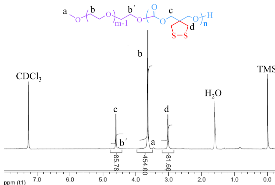
Fig. 2. ^1\text{H} NMR spectrum (400 MHz, \text{CDCl}_3 ) of PEG- b -PDTC diblock copolymer.
