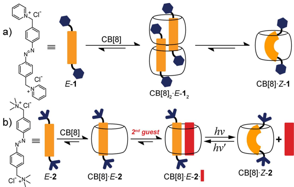
Formation of host-guest complexes of CB[8] with 1 (a), and stepwise formation of 1:1:1 ternary complex of CB[8] with E-2 and second guest molecule followed by light induced release (b). 84x52mm (300 x 300 DPI)
