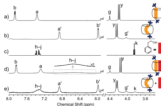
Figure 3. Selected regions of the 1 H NMR spectra (500 MHz, D 2 O, 298 K) of (a, b) CB[8]· 2 before (a) and after (b) UV light irradiation, 4 (c), and (d, e) CB[8]· E - 2 · 4 before (d) and after (e) UV light irradiation. See Chart 1 for proton labeling. Signals corresponding to protons of Z - 2 are indicated with apostrophes.
