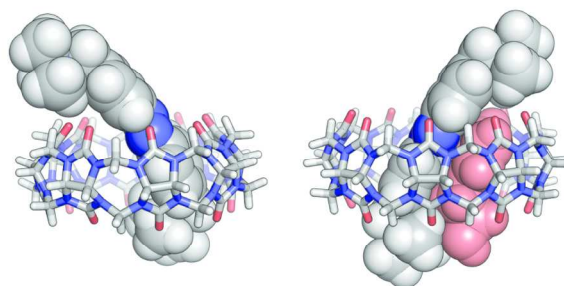
Geometry-optimized molecular structures (M062X/6-31G* level of theory) of CB[8]• E - 2 (left) and CB[8]• E - 2•4 (right) complexes. 144x49mm (300 x 300 DPI)
