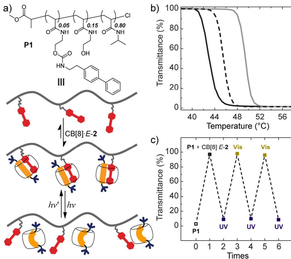
Structure of P1 and schematic representation of the light-controlled complexation of the biphenyl moieties of P1 (a). Transmittance (recorded at 600 nm and at a heating rate of 1 °C/min) of P1 (0.1 mM in H 2 O) as a function of temperature (b) in the absence (full black line) and presence (full gray line) of CB[8]•E-2, and after UV light irradiation (dashed line). Changes in the transmittance of P1 (0.1 mM in H 2 O) at 47 °C by alternating irradiation with UV and visible light in the presence of CB[8] and 2 (c).
