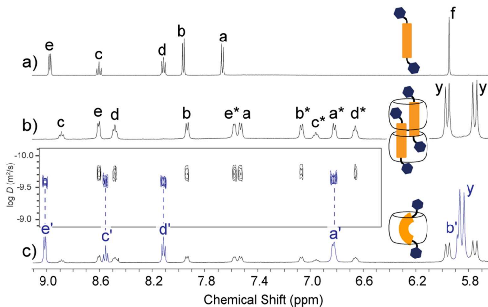
Partial ^1\text{H} NMR spectra (500 MHz, \text{D}_2\text{O} , 298 K) of E - 1 (a), a freshly prepared solution of an equimolar mixture of CB[8] and E - 1 (b) and after storage in the dark at 298 K for ~3 months (c) and corresponding ^1\text{H} DOSY plots. Signals corresponding to Z - 1 protons in (c) are indicated with apostrophes. The two groups of ^1\text{H} NMR signals of the asymmetrically encapsulated E - 1 in (b) are denoted by \text{H}_\alpha\text{-e} and \text{H}_\alpha^*\text{-e}^* (see Chart 1 for proton labeling and text for more details).
