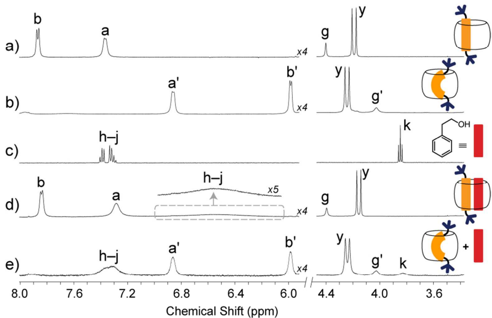
Selected regions of the 1 H NMR spectra (500 MHz, D 2 O, 298 K) of (a, b) CB[8]• 2 before (a) and after (b) UV light irradiation, 4 (c), and (d, e) CB[8]• E-2•4 before (d) and after (e) UV light irradiation. See Chart 1 for proton labeling. Signals corresponding to protons of Z-2 are indicated with apostrophes
