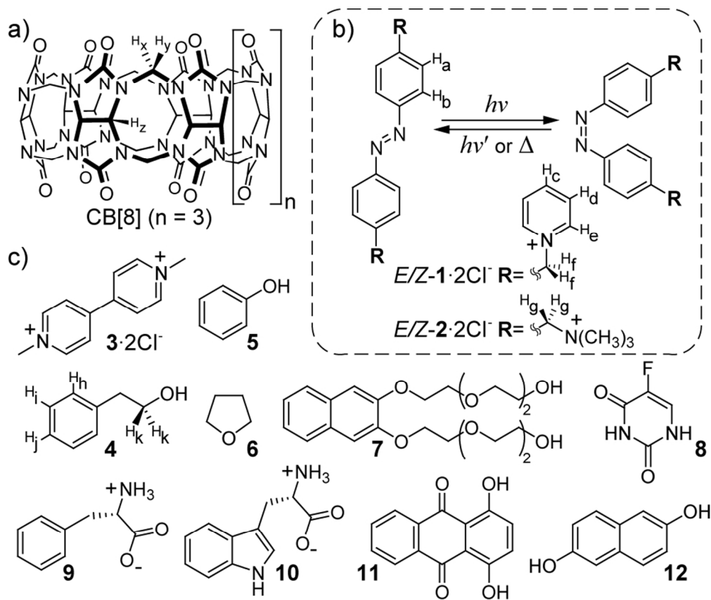
Structures of CB[8] (a), photoresponsive first guests molecules 1 and 2 (b) and selected guests 3-12 (c). 83x71mm (300 x 300 DPI)
