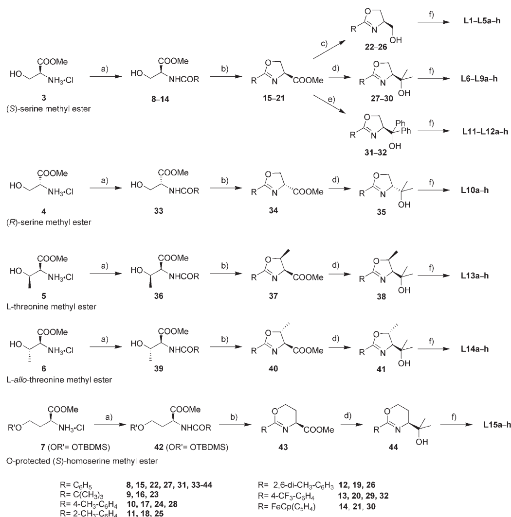
Scheme 2. Synthesis of phosphite-oxazoline and phosphite-oxazine ligand library L1-L15a-h . a) \text{RCOCl}/\text{NEt}_3/\text{CH}_2\text{Cl}_2 (yields 85–99%). b) \text{DAST}/\text{CH}_2\text{Cl}_2 (yields 86–98%). c) \text{LiAlH}_4/\text{Et}_2\text{O} (yields 79–94%). d) \text{CH}_3\text{MgCl}/\text{Et}_2\text{O}/\text{THF} (yields 81–96%). e) \text{PhMgCl}/\text{Et}_2\text{O}/\text{THF} (yields 84–93%). f) \text{CIP}(\text{OR})_2 ; (OR) 2 = a-h /Py/toluene (yields 34–81%).
