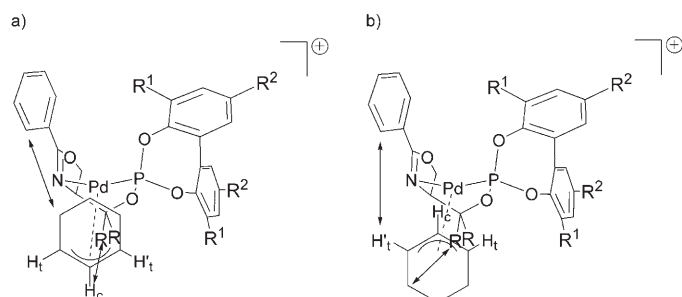
Figure 8. Relevant NOE contacts from NOESY experiment for a) isomers A and b) isomers B of complexes [\text{Pd}(\eta^3\text{-1,3-cyclohexenylallyl})\text{-(L6c)}]\text{BF}_4 ( 61 ; \text{R}=\text{Me} , \text{R}^1=\text{SiMe}_3 and \text{R}^2=\text{H} ) and [\text{Pd}(\eta^3\text{-1,3-cyclohexenylallyl})\text{-(L11a)}]\text{BF}_4 ( 62 ; \text{R}=\text{Ph} , \text{R}^1=\text{R}^2=\text{tBu} ).
