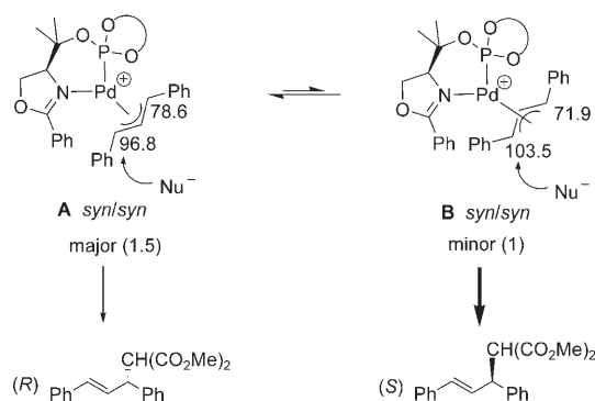
Scheme 4. Diastereoisomer Pd-allyl intermediates for 51 with ligand L6a . The relative amounts of each isomer are drawn in parenthesis. The chemical shifts (in ppm) of the allyl terminal carbons are shown.
