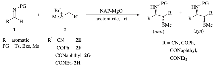
Scheme 2. NAP-MgO catalyzed Mannich-type reaction between N -sulfonyl aldimines 1 and nitrile/ketone/amide sulfonium salts 2E–H .
