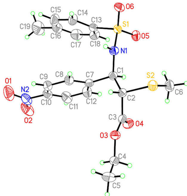
Figure 1. Thermal ellipsoidal plot of compound ethyl-3-[[[(4-methylphenyl)sulfonyl]amino]-2-(methylsulfanyl)-3-(4-nitrophenyl)propanoate (major isomer) (Table 3, entry 3). Displacement ellipsoids are drawn at the 25% probability level except for the hydrogen atoms, which are shown as circles of arbitrary radius.
