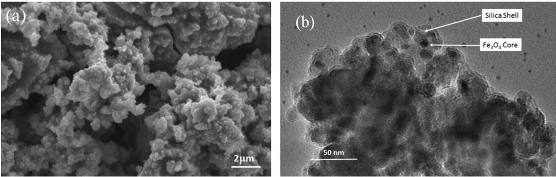
Figure 2: (a) SEM and (b) TEM images of Fe 3 O 4 @SiO 2 -SO 3 H catalyst.
