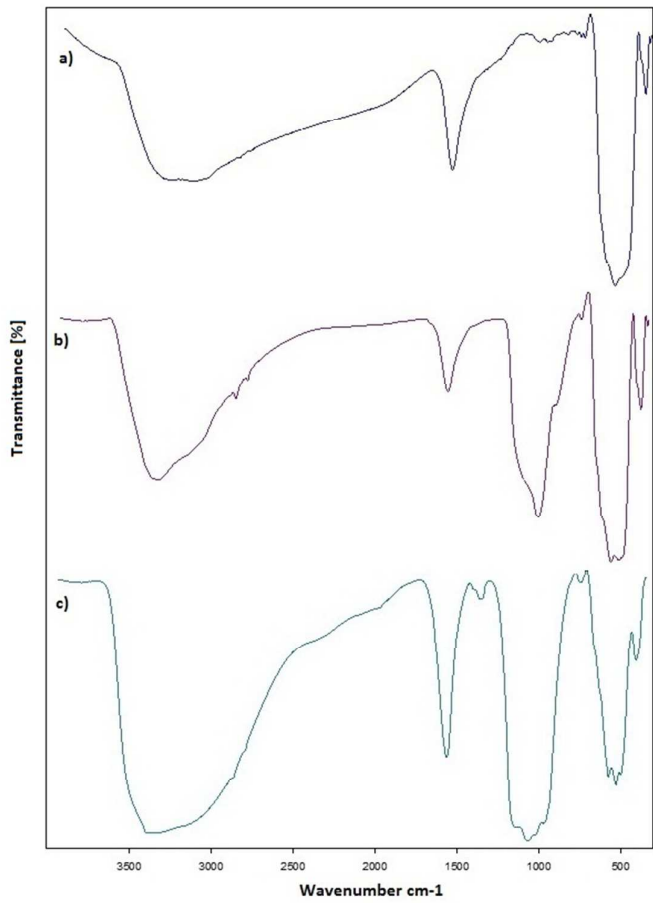
Figure 6: FT-IR spectra of (a) Fe 3 O 4 , (b) Fe 3 O 4 @SiO 2 and (c) Fe 3 O 4 @SiO 2 -SO 3 H.
