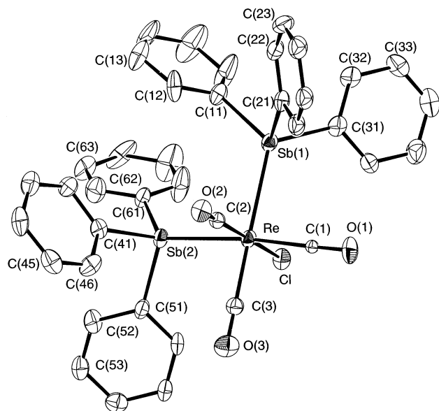
Fig. 3. Molecular structure of [\text{Re}(\text{CO})_3\text{Cl}(\text{SbPh}_3)_2] showing the atom labeling scheme. Displacement ellipsoids are drawn at the 50% probability level and H atoms are excluded for clarity.
