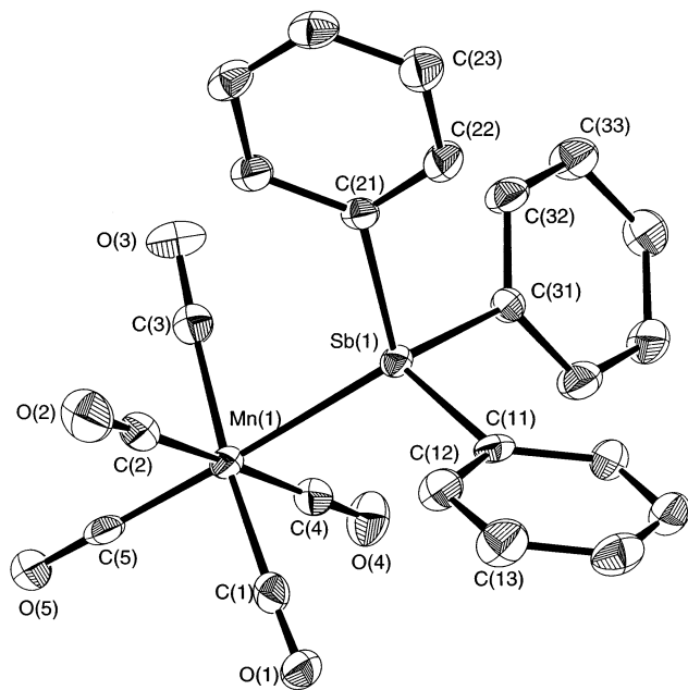
Fig. 2. Structure of the cation in [\text{Mn}(\text{CO})_5(\text{SbPh}_3)][\text{CF}_3\text{SO}_3] showing the atom labeling scheme. Displacement ellipsoids are drawn at the 50% probability level and H atoms excluded for clarity.
