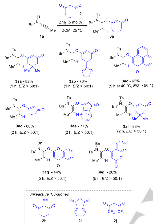
Scheme 2. Scope investigation of the \text{ZnI}_2 -catalyzed addition with various 1,3-diones.
