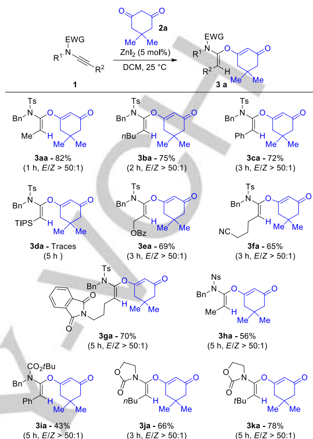
Scheme 3. Scope investigation with various internal ynamides (Ns = \text{SO}_2(p\text{-NO}_2\text{-C}_6\text{H}_4) ).
