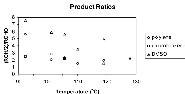
FIGURE 7. Ratio of the integration of p -nitrobenzyl alcohol 3a to p -nitrobenzaldehyde 4a per mole of integratable protons.
