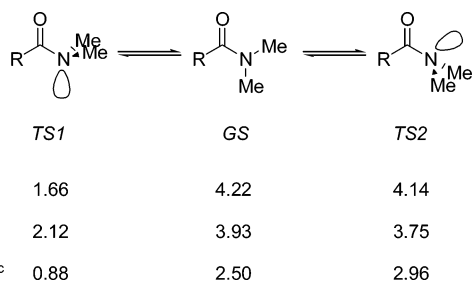
FIGURE 5. Gas-phase ground- and transition-state dipoles (D) for amide and carbamate isomerization. (a) Dipole moments calculated at HF/6-31++G**. Here, rotation through TS1 is preferred by 3.5 kcal/mol. 37 (b) Dipole moments calculated at HF/6-31G*. Here, TS1 is to be more stable than TS2 by 4.1 kcal/mol. 39 (c) Dipole moments calculated at HF/6-311G**. Here, TS1 is more stable than TS2 by 0.6 kcal/mol. 44
