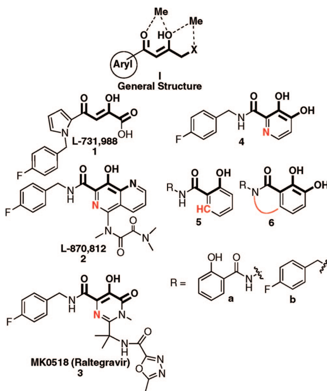
Figure 1. Structural features of a general IN inhibitor (I) common to diketo acid ( 1 ) and later generation inhibitors.
