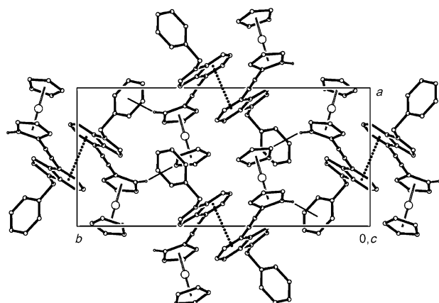
Figure 4. A drawing of the unit cell of 3a as viewed along the crystallographic c axis. The most important intermolecular interactions are highlighted: \pi\cdots\pi stacking as dotted lines and C–H \cdots\pi interactions as solid lines.
