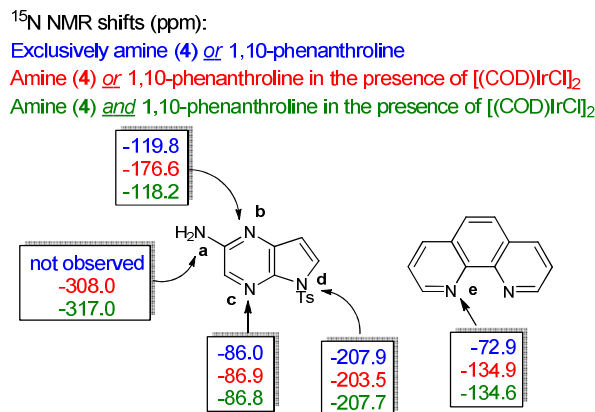
Figure 2. Interaction of [(\text{COD})\text{IrCl}]_2 with amine ( 4 ) and 1,10-phenanthroline as studied by ^1\text{H} - ^{15}\text{N} HMBC spectroscopy.
