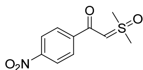
2-(Dimethyl(oxo)-λ 6 -sulfanylidene)-1-(4-nitrophenyl)ethan-1-one
