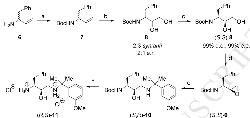
Scheme 1. Synthesis of amino alcohol intermediate ( R,S )- 11 . Reagents and conditions: a) \text{Boc}_2\text{O} (1.25 equiv), \text{NEt}_3 (2 equiv), DCM, rt, 2 h, 87%. b) AD-mix- \alpha (1 equiv), 1:1 (v/v) t -BuOH:water, rt, 20 h. c) preparative HPLC on chiral stationary phase ( Chiralpack-ID ), 25% in two steps. d) \text{Ph}_3\text{P} (1.1 equiv), DEAD (1.1 equiv), \text{CHCl}_3 , 85 °C, 48 h, 64%. e) 2-(3-Methoxyphenyl)propan-2-amine 11 (1.05 equiv), i -PrOH, 70 °C, 40 h, 73%. f) 4 M HCl in dioxane, rt, 6h, 99%.
