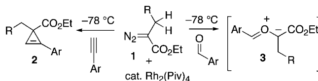
Scheme 1. Intermolecular Reactions without \beta -Hydride Elimination
