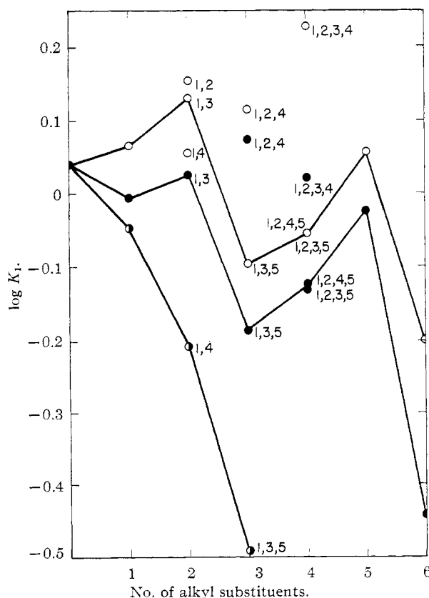
Fig. 1.—Variations in \log K_1 with the number of alkyl substituents on the benzene ring: O, methylbenzenes; ●, ethylbenzenes; ●, t -butylbenzenes.
