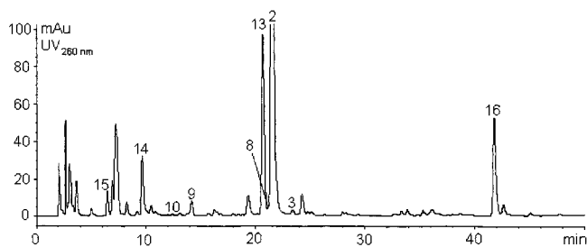
Figure 4. HPLC–UV/MS chromatogram obtained from a model wine solution spiked with 2 directly after sulfuration ( 2 , indole-3-acetic acid; 3 , 2-aminoacetophenone; 8 , 2-formamidoacetophenone; 9 , 2-oxindole-3-acetic acid; 10 , 3-(2-formylaminophenyl)-3-oxopropionic acid; 13 , indole-3-aldehyde; 14 , (2-sulfoindole)-3-acetic acid; 15 , 2,3-dioxindole-3-acetic acid; 16 , 2-(3-indolylmethyl)-indole-3-acetic acid). Quantification of 8 was possible only by evaluation of its MS signal.
