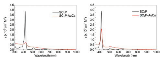
Figure 3. UV-vis-NIR spectra for SC n P and SC n P–AuCs in DMF. The extinction coefficients of SC n P on SC n P–AuCs were estimated from inductively coupled plasma atomic emission spectroscopy data.
