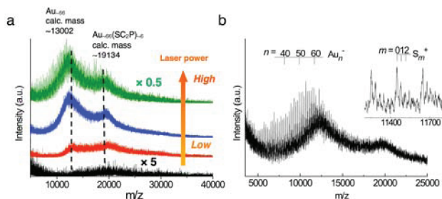
Figure 4. (a) MALDI-TOF mass spectra of \text{SC}_2\text{P-AuCs} at various laser powers. (b) MALDI-TOF mass spectra of \text{SC}_2\text{P-AuCs} at high laser power. Regular progressions of the mass spectra, which correspond to Au and sulfur atoms, were observed. The inset shows the expanded image of progressions of \text{Au}_n^- and \text{Au}_n\text{S}_m^- ( m \geq 1 ).
