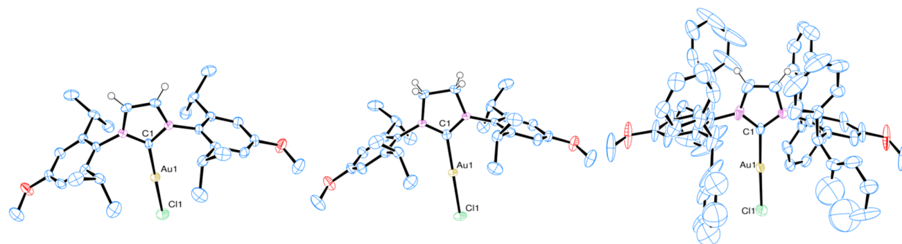
Figure 1. X-ray crystal structures of (left) [\text{AuCl}(\text{IPr}^{\text{OMe}})] ( 1b ), (center) [\text{AuCl}(\text{SIPr}^{\text{OMe}})] ( 1d ), and (right) [\text{AuCl}(\text{IPr}^{\ast\text{OMe}})] ( 1f ). Thermal ellipsoids are drawn at the 50% probability level, and most H atoms are excluded for clarity.
