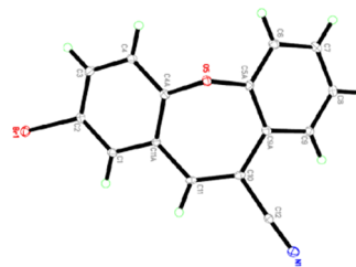
X-ray structure of 10b
