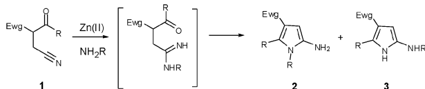
Scheme 1 Zn(II) salt catalyzed formation of pyrroles.
