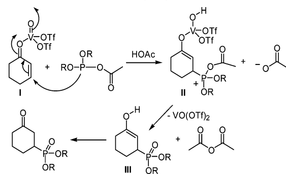
Scheme 2. Proposed Mechanism for Phospha-Michael Addition of an Acetylphosphite to an Enone Catalyzed by VO(OTf) 2
