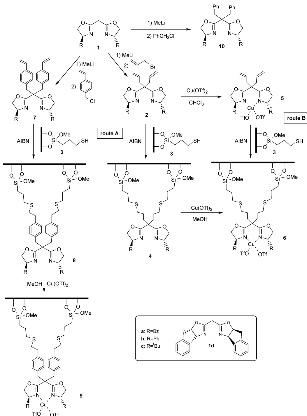
Scheme 1. Immobilization of Bis(oxazoline)copper Complexes onto Silica
