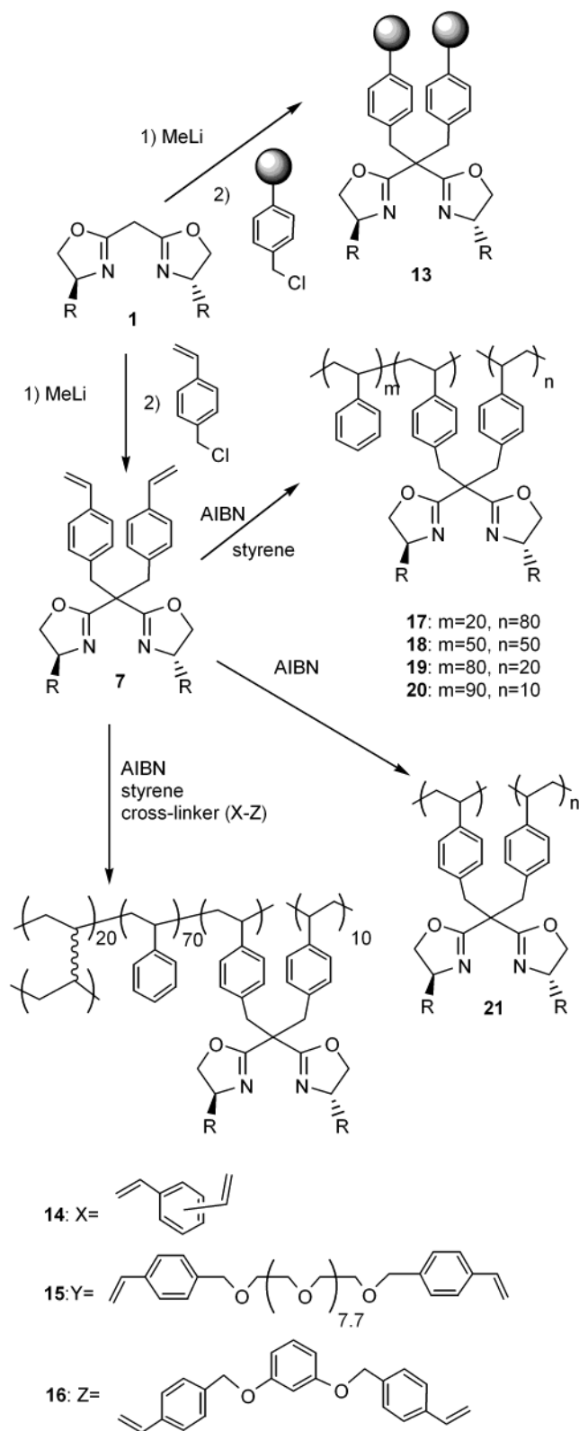
Scheme 3. Preparation of Polymeric Bis(oxazoline) Ligands by Grafting and Polymerization
