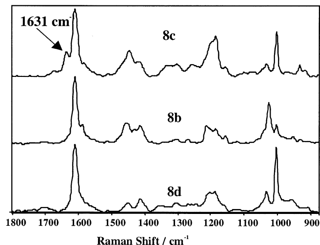
Figure 2. Raman spectra of solids 8b – d .
