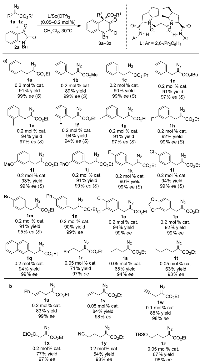
Scheme 2. Scope of \alpha -alkyl- \alpha -diazoesters in the catalytic asymmetric ring expansion. The reactions were performed with L /Sc(OTf) 3 (0.05–0.2 mol %, 1:1.2), 2a (0.20 mmol), 1 (0.30 mmol), CH 2 Cl 2 (0.2 mL) in 30 °C for 5–50 h (for details, see the Supporting Information). Yields of isolated products are reported. The ee values were determined by HPLC using a chiral stationary phase. The absolute configuration of 3a was determined to be S by X-ray crystallographic analysis, and those of 3b–3m were assigned by comparing their circular-dichroism spectra with that of 3a . TBS = tert -butyldimethylsilyl, Tf = trifluoromethanesulfonyl.
