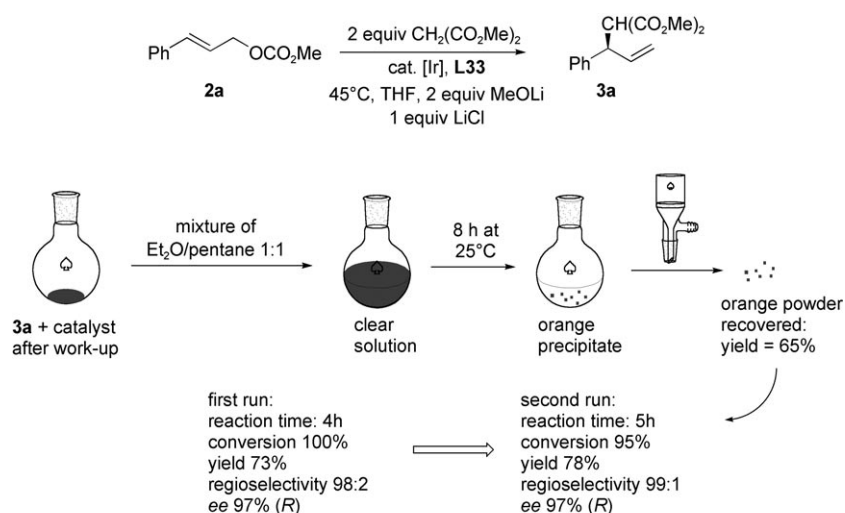
Scheme 16. Catalyst recycling technique.
