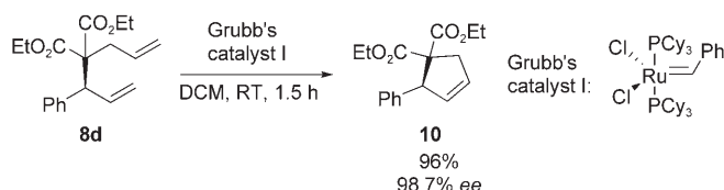
Scheme 9.
