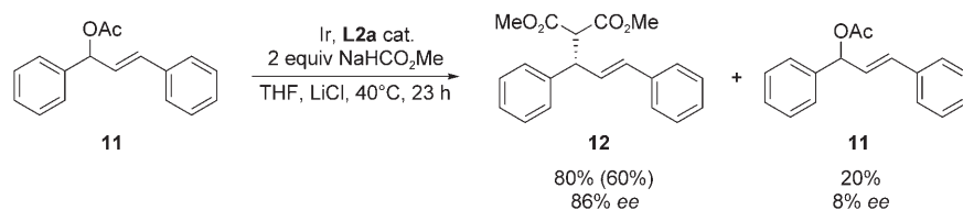
Scheme 13.
