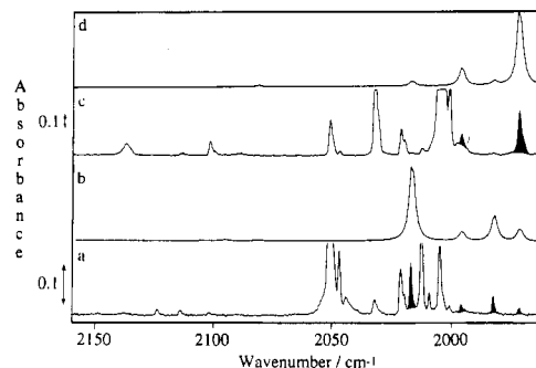
Figure 2. Stacked plot comparing the IR spectrum observed for \text{Ni}(\text{CO})_3 in the region 1960–2160 cm −1 (bands marked by black in-filling) with that predicted on the basis of a planar tricarbonyl of D_{3h} symmetry with the force constants given in Table 1: (a) observed and (b) predicted for 27% 13 CO-enrichment; (c) observed and (d) predicted for 82% 13 CO-enrichment.
