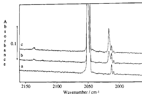
Figure 1. IR spectrum of \text{Ni}(\text{CO})_4 isolated in an Ar matrix ( \text{Ar}:\text{Ni}(\text{CO})_4 = \text{ca. } 1:2000 ) in the region 1960–2160 cm −1 : (a) after deposition; (b) after 60 min of photolysis at ca. 254 nm; (c) after 120 min of broad-band photolysis.
