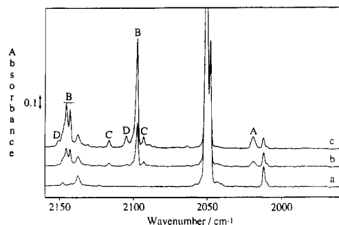
Figure 3. IR spectrum of \text{Ni}(\text{CO})_4 isolated in an \text{O}_2 -doped Ar matrix ( \text{Ar}:\text{O}_2:\text{Ni}(\text{CO})_4 = 1500:150:1 ) in the region 1960\text{--}2160\text{ cm}^{-1} , showing the effects of photolysis at wavelengths near 254\text{ nm} : (a) after deposition; (b) after 60 min of photolysis; (c) after 180 min of photolysis.
