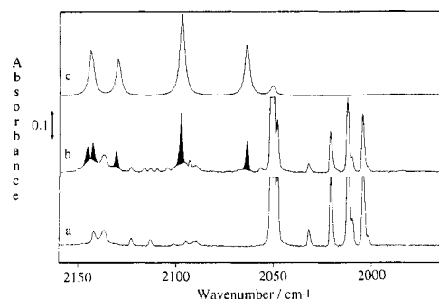
Figure 4. Stacked plot comparing the IR spectrum in the region 1960\text{--}2160\text{ cm}^{-1} observed for B with 27\% ^{13}\text{CO} -enrichment (bands marked by black in-filling) with that predicted on the basis of a bent dicarbonyl fragment with the geometry and force constants given in Table 2: (a) on deposition; (b) after 60 min of photolysis at ca. 254\text{ nm} ; (c) simulated spectrum.
