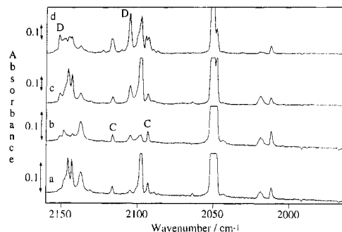
Figure 9. IR spectrum of \text{Ni}(\text{CO})_4 isolated in an \text{O}_2 -doped argon matrix ( \text{Ar}:\text{O}_2:\text{Ni}(\text{CO})_4 = 1500:150:1 ) in the region 1960\text{--}2160\text{ cm}^{-1} : spectrum of sample (a) after 60 min of photolysis at ca. 254\text{ nm} following deposition and (b) after a further 80 min of photolysis at 313\text{ nm} ; spectrum of separate sample (c) after 360 min of photolysis at ca. 254\text{ nm} following deposition and (d) after annealing the deposit to approximately 30\text{ K} .
