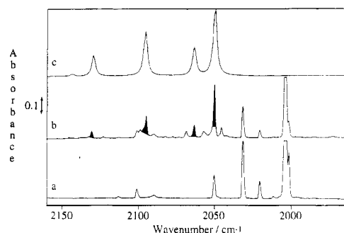
Figure 5. Stacked plot comparing the IR spectrum in the region 1960\text{--}2160\text{ cm}^{-1} for B with 82\% ^{13}\text{CO} -enrichment (bands marked by black in-filling) with that predicted on the basis of a bent dicarbonyl fragment with the geometry and force constants given in Table 2: (a) on deposition; (b) after 60 min of photolysis at ca. 254\text{ nm} ; (c) simulated spectrum.
