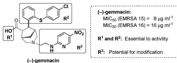
Fig. 1 (–)-Gemmacin showed good activity against EMRSA 15 and 16 (MIC 50 values of 8 and 16 µg ml –1 respectively), and was shown to be a selective bacterial cell membrane disrupter. When R 1 and/or R 2 were altered, the resulting compounds were no longer active ( i.e. MIC 50 > 64 µg ml –1 ). R 3 served as the site for SAR investigation in this report.
