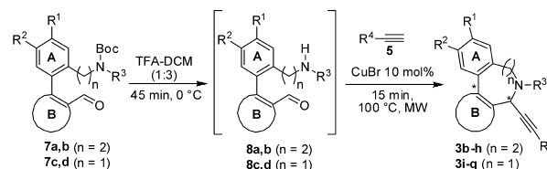
Scheme 2. Investigation of the Scope of the Intramolecular A 3 -Coupling Reaction
