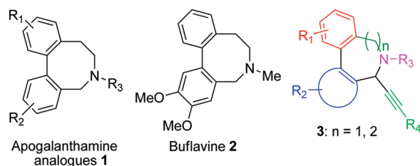
Figure 1. Structure of the apogalanthamine analogues (1), bufavine (2), and the proposed new analogues 3.
