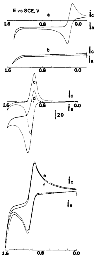
Figure 8. Cyclic voltammetry in 0.1 M KCl at 10 mV/s: (a) \text{SnO}_2 electrode in 1 mM \text{K}_4\text{Fe}(\text{CN})_6 ; (b) \text{SnO}_2/\text{NAF} ( d = 0.4 \mu\text{m} ) in 1 mM \text{K}_4\text{Fe}(\text{CN})_6 ; (c) \text{SnO}_2/\text{NAF} , \text{Ru}(\text{bpy})_3^{2+} in base electrolyte ( d = 0.3 \mu\text{m} ); (d) same electrode as (c) with 1 mM \text{K}_4\text{Fe}(\text{CN})_6 added to the solution; (e) \text{SnO}_2/\text{NAF} , \text{Ru}(\text{bpy})_3^{2+} thick film electrode in base electrolyte; (f) same electrode with 1 mM \text{K}_4\text{Fe}(\text{CN})_6 added to the solution.
