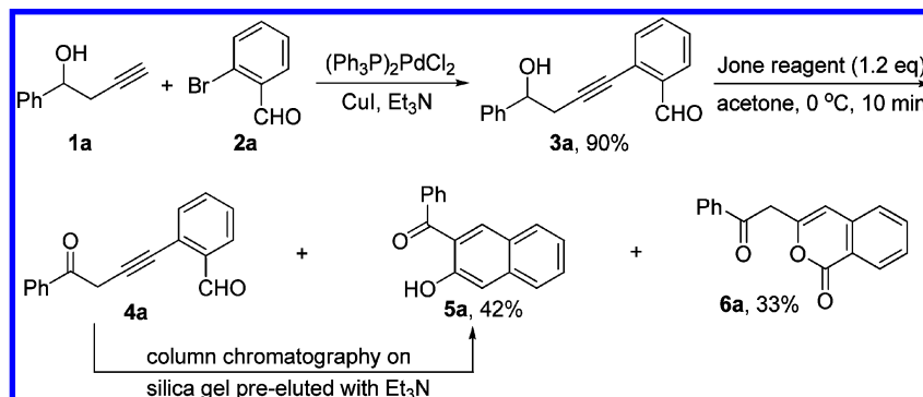
Scheme 2. Unexpected Formation of 5a and 6a from the Reaction of 3a
