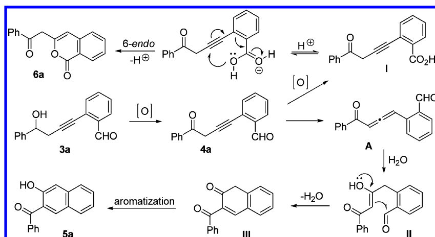
Scheme 4. Plausible Mechanism for the Formation of 5a and 6a from 3a
