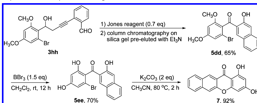
Scheme 5. Alternative Synthetic Pathway toward Compound 7
